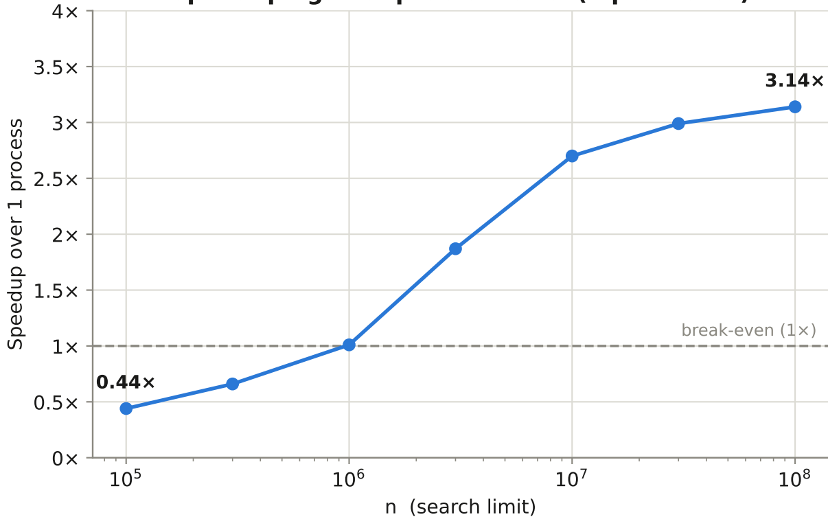
Speedup against problem size (4 processes)
